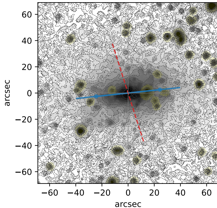
S4G 3.6 micron isophotes
