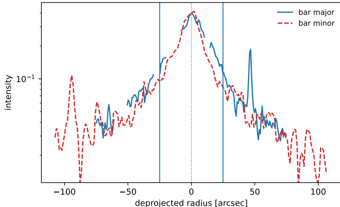
major/minor-axis cuts (35308 masked px ignored)
